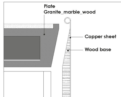
Detail
