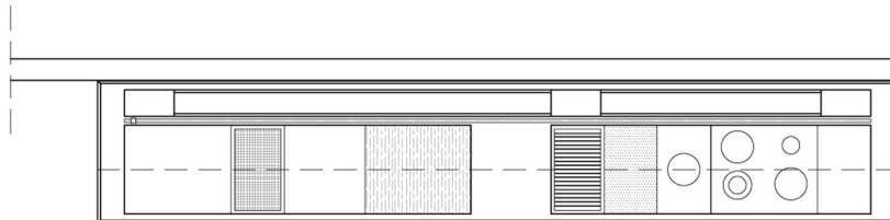
Kitchen in-line
