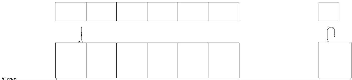
Views
