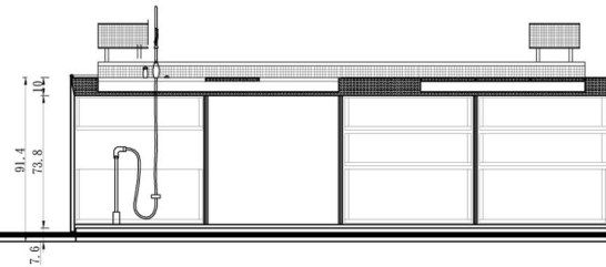
Sections
