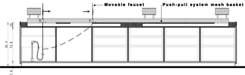
Sections
